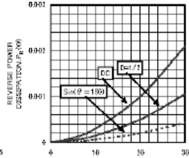
REVERSE VOLTAGE V_R (V) VR-P c CHARACTERISTICS
