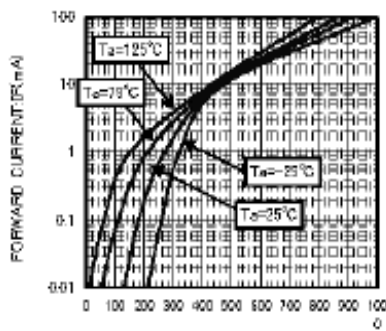
FORWARD VOLTAGE: V F (mV) VF-IF CHARACTERISTICS VF分布
