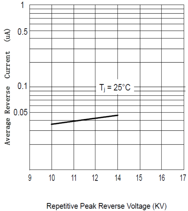
REVERSE CHARACTERISTIC [VR-IR]
