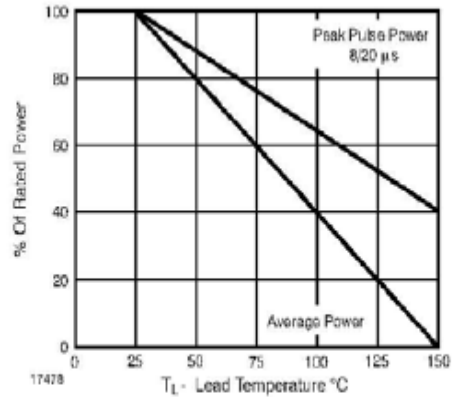
Figure 3. Power Derating
