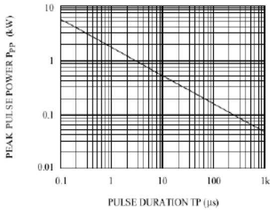
NON-REPETTITIVE PEAK PULSE POWER VS. PULSE TIME
