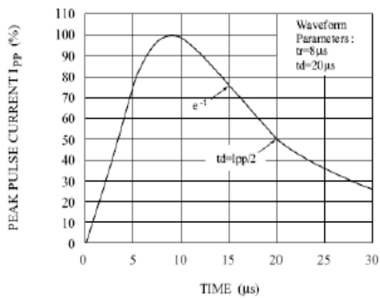
PULSE WAVEFORM
