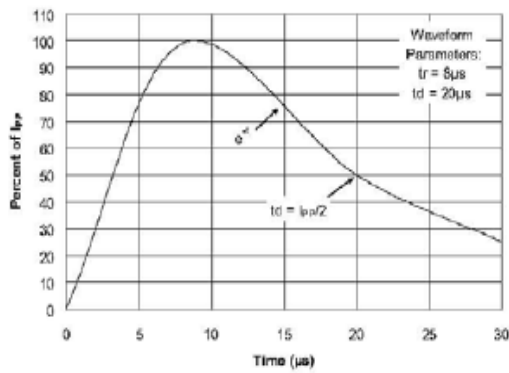
Pulse Waveform
