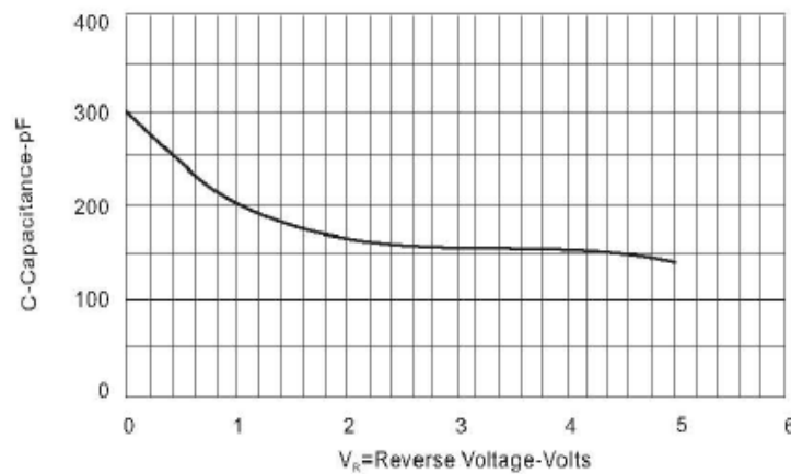
FIG.4-Typical Reverse Voltage vs Capacitance
