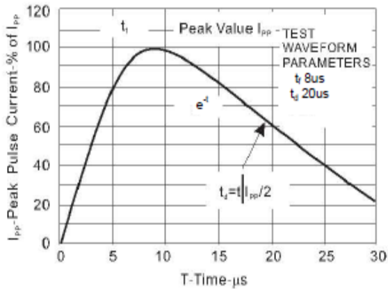
FIG.1-Pulse Wave Form
