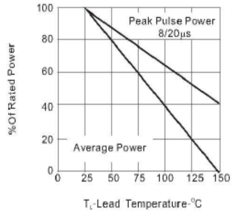
FIG.2-Power Derating Curve
