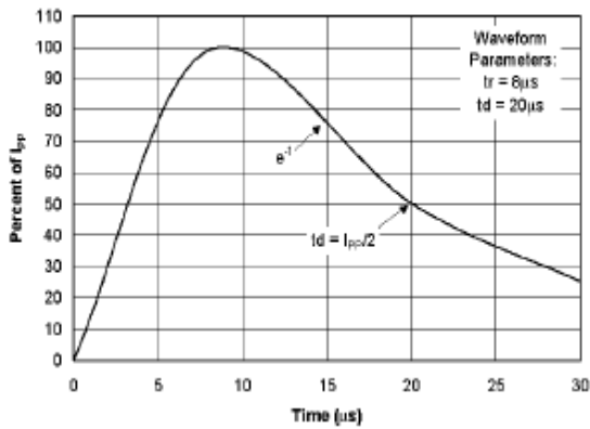
Pulse Waveform
