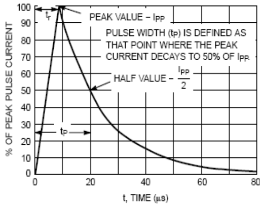
Figure 1. 8 x 20 \mu s Pulse Waveform
