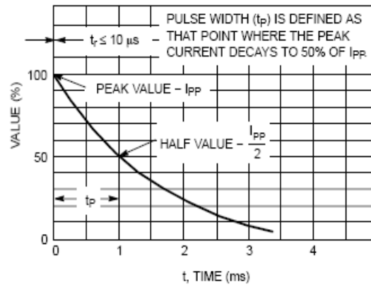
Figure 2. 10 x 1000 \mu s Pulse Waveform
