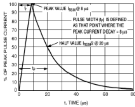
Figure 1. 8 x 20 \mu s Pulse Waveform
