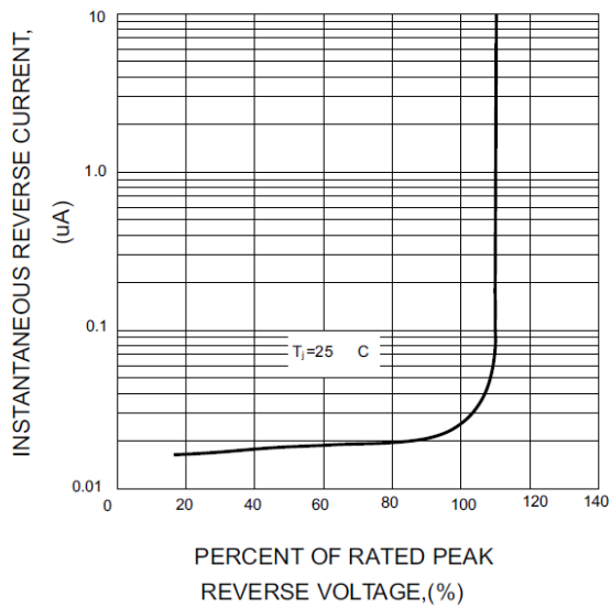
FIG.3-TYPICAL REVERSE CHARACTERISTICS
