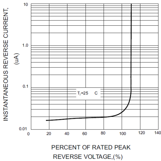
FIG.3-TYPICAL REVERSE CHARACTERISTICS
