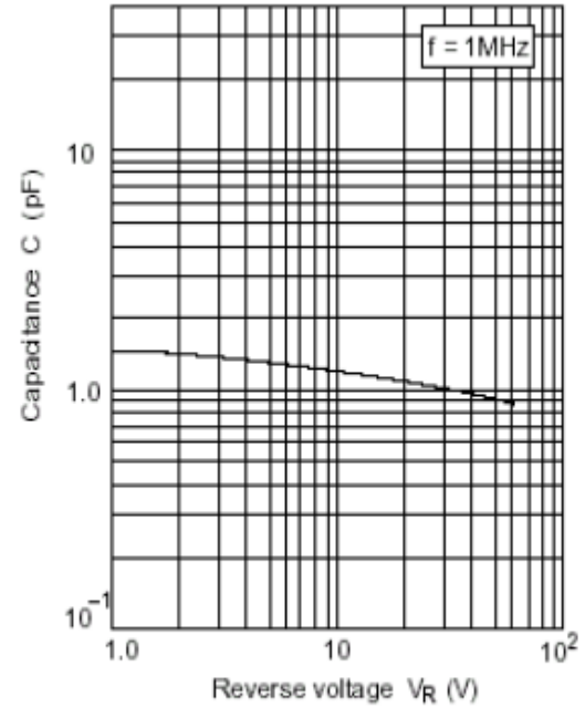
Capacitance Vs. Reverse voltage
